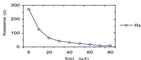
Fig.1 Resistance Rx as a function of IDN3
